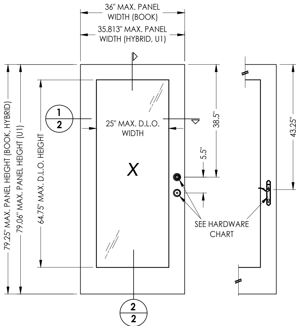
40 DOOR PANEL Classic-Craft Shaker
